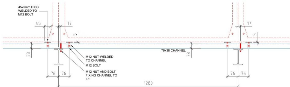
LEVELING BEAM DETAIL SCALE 1:10
