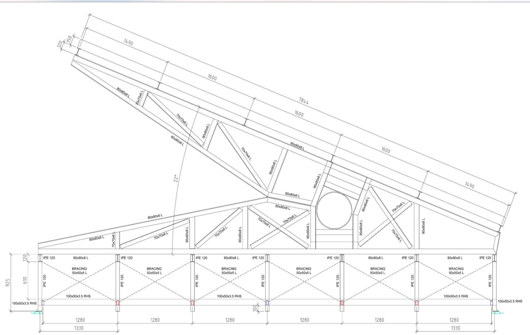
PLAN ON TYPICAL HORIZONTAL TRUSS SCALE 1:25
