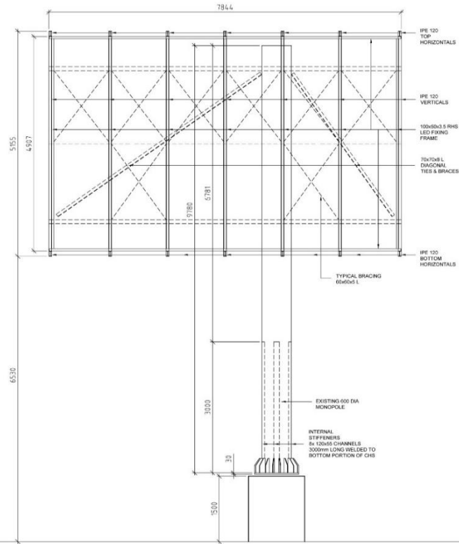
FRONT ELEVATION ON BILLBOARD STRUCTURE SCALE 1:75
