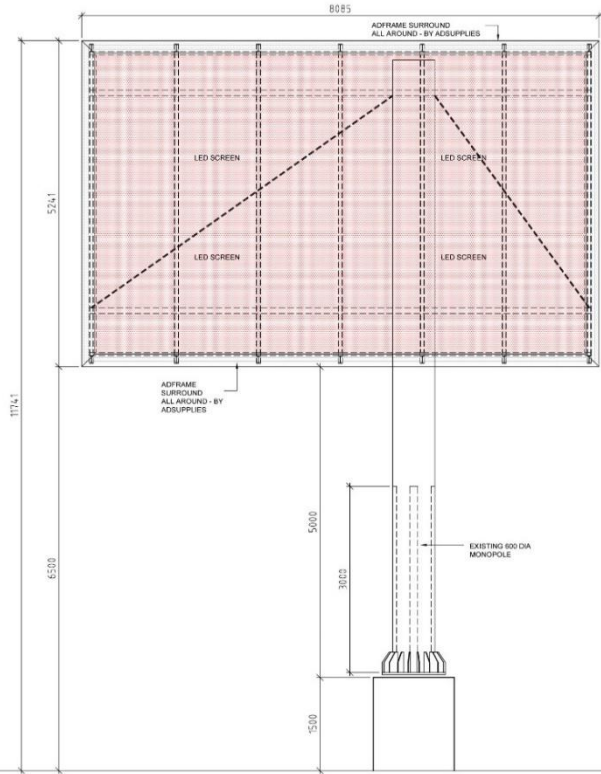
ELEVATION ON LED BILLBOARD SCALE 1:75
